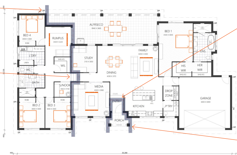
SIDE-TO-SIDE SPLIT Georgia 311 with 3 Level Split
